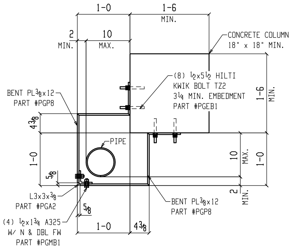
PIPE GUARD PG8 @ COLUMN
