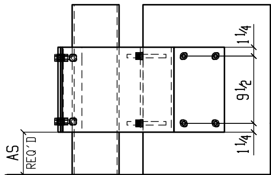
PIPE GUARD PG8 @ COLUMN
